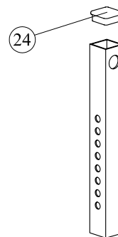
I.ASSY,ADJUSTING TUBE
