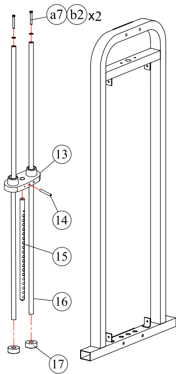
A.ASSY,WEIGHT SIDE FRAME F.ASSY, TOP WEIGHT
