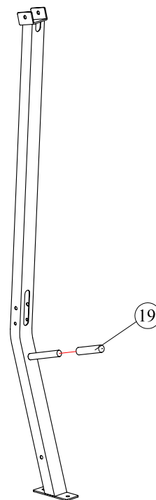
C.ASSY,FRONT UPRIGHT
