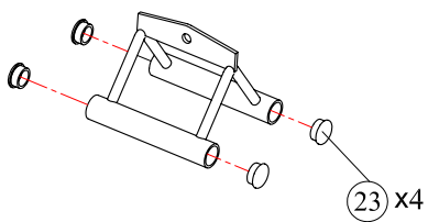
H.ASSY,LOW ROW "V" BAR
