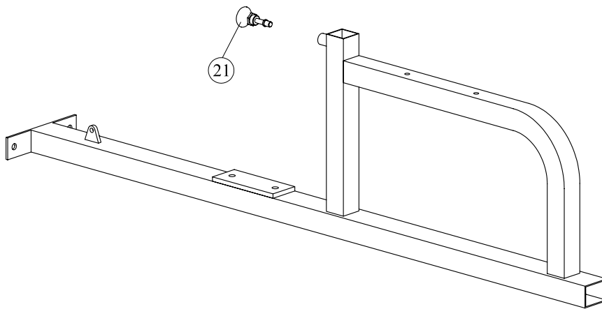
E.ASSY,SEAT FRAME
